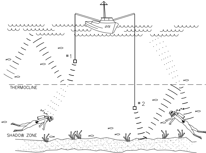
Figure 13: Thermoclines affect the ultrasonic signal. Divers must report thermocline depth(s) so the surface transceiver and/or other divers can be as close to the same depth as possible.
