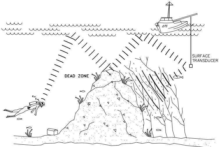
Figure 15: Communication through indirect and direct paths. Note help scattering sound. Without surface and bottom bounce, the diver would lose communications.
